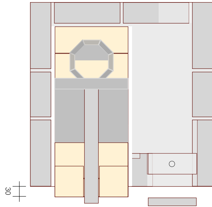
9. Placing the core, the joining brick and the buffer
