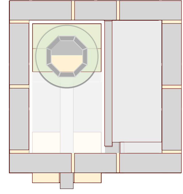
12. Insulation, upper part riser, layers 5 - 7
